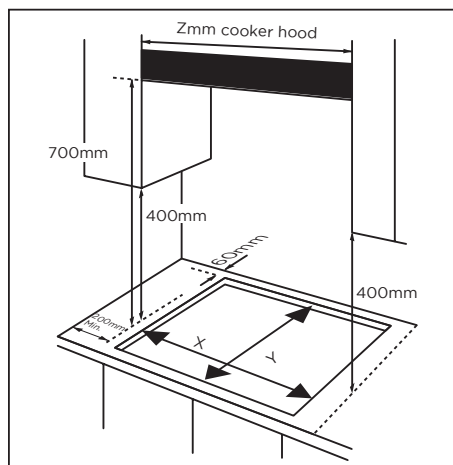
CLEARANCES REQUIRED WHEN FITTING THE HOB WITH A COOKER HOOD ABOVE
